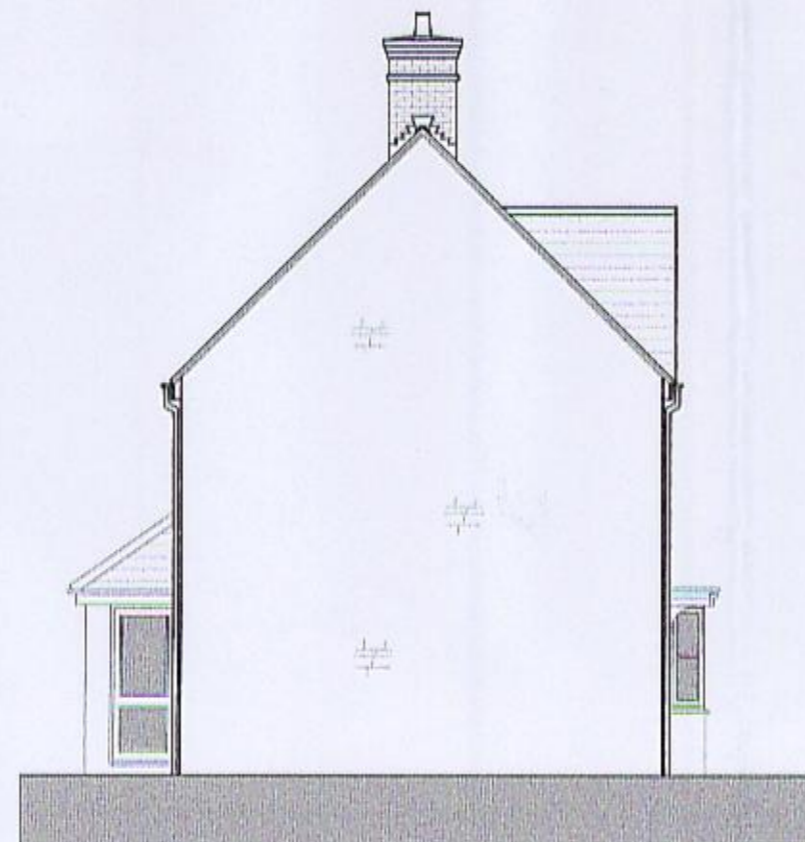
SIDE ELEVATION TYPE J2 - IRON STONE PLOTS 67, 73 & 86
