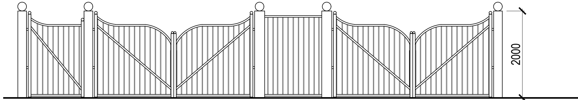
Proposed elevation—entrance gate
