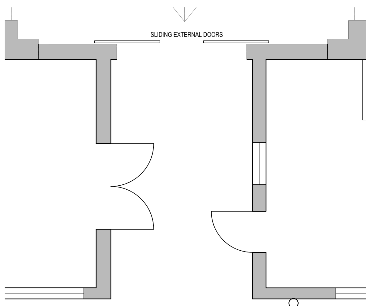
04 EXISTING PLAN 1:50
