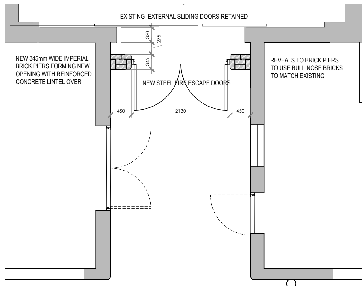
01 PROPOSED PLAN 1:50
