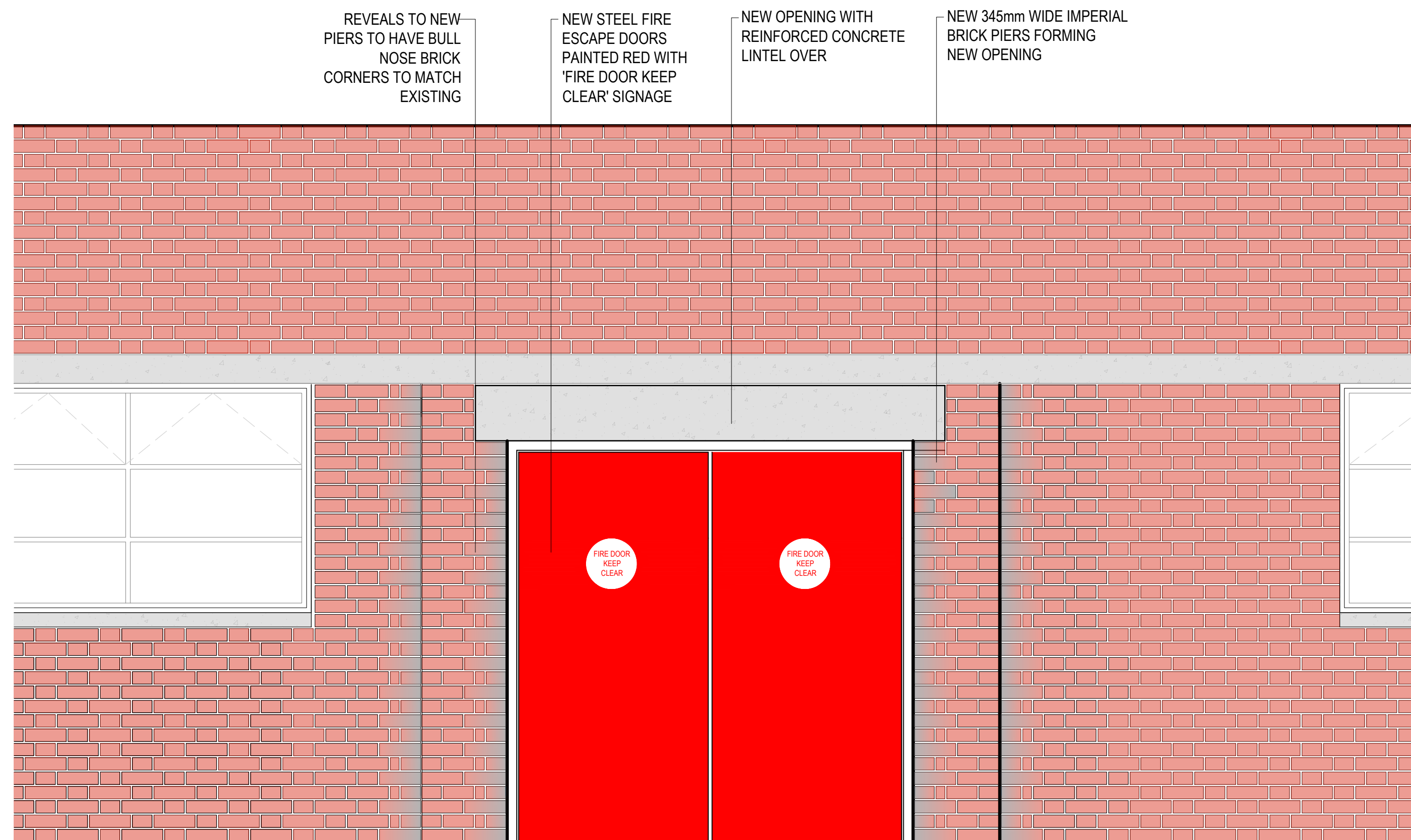
06 PROPOSED DOOR ELEVATION 1:20
