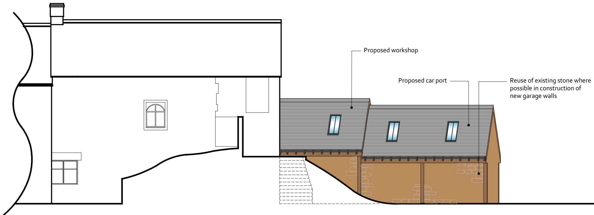
Proposed North Elevation Scale 1:100
