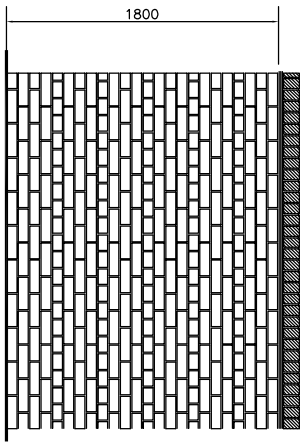
1800mm HIGH SCREEN WALL
