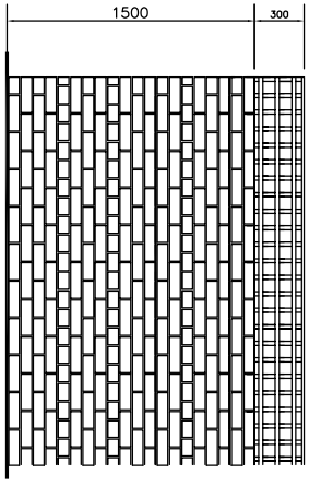
1500mm HIGH DWARF WALL WITH 300mm HIGH TRELLIS
