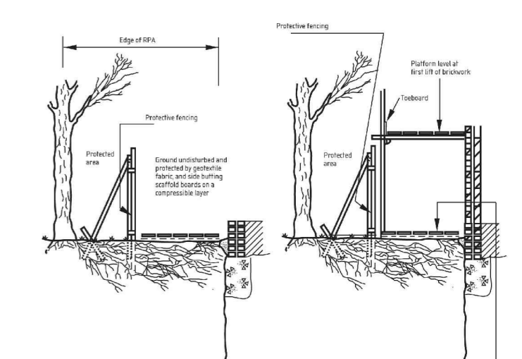
Diagram 2: Scaffolding within the root protection area, to British Standard 5837:2012 Trees in relation to construction
