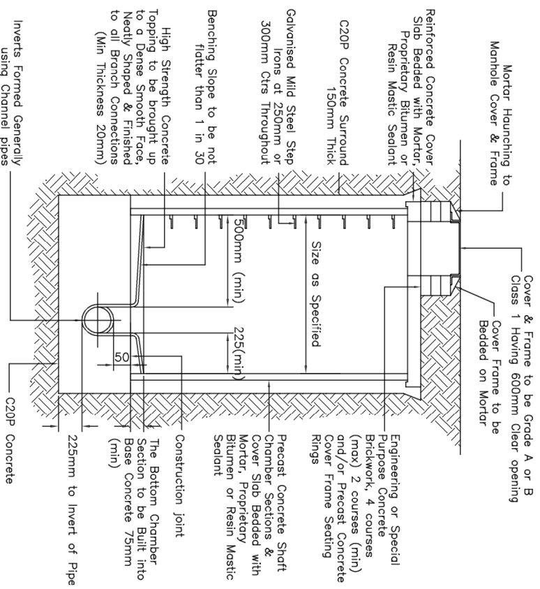
TYPICAL MANHOLE 1:20
