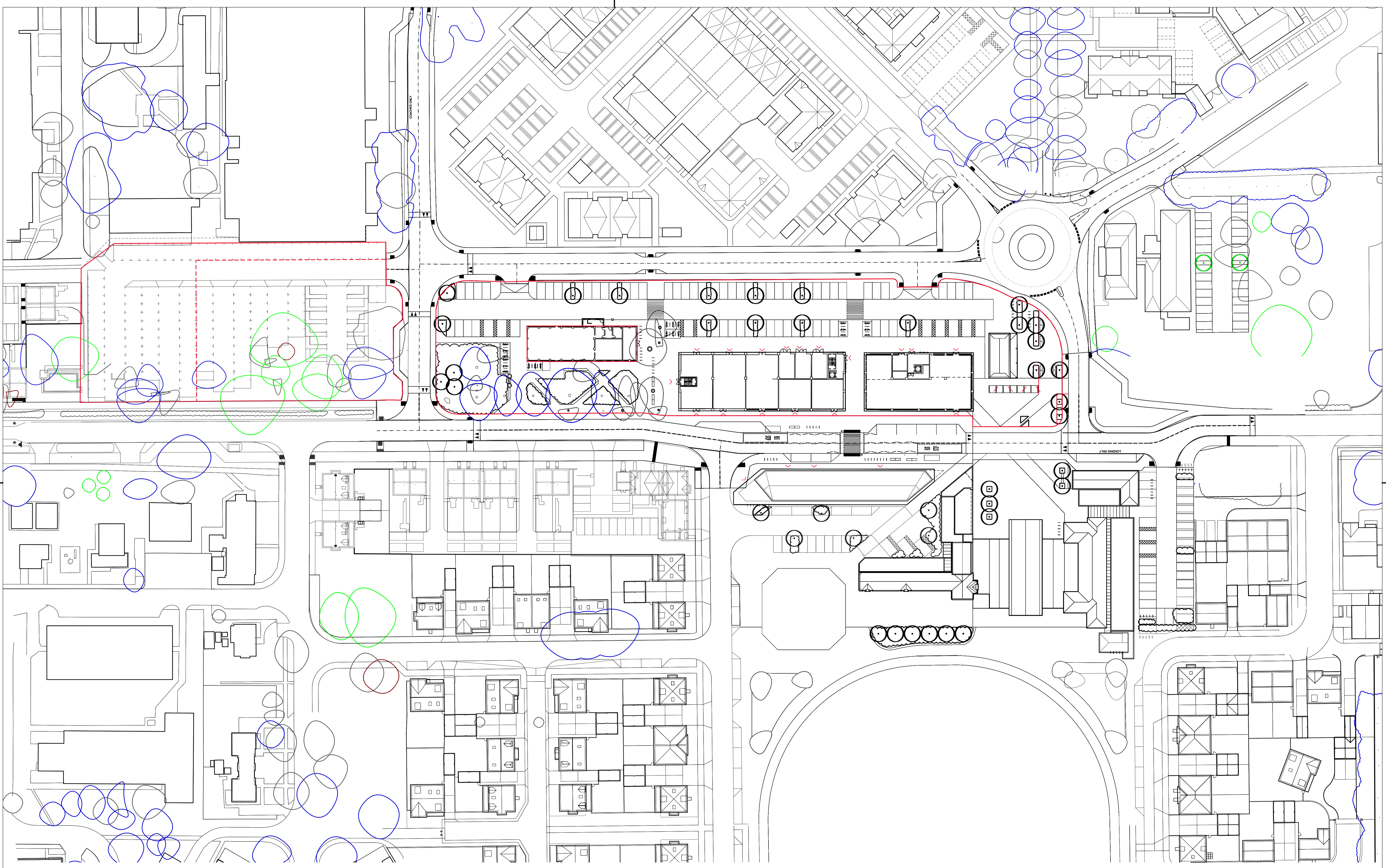
Heyford Park Village Centre - Northern Plot General Arrangement Plan Eden Development Consultants - 16/03/2018 - EDC05-GA-100 - Rev J Drwn by: RDG - Scale 1:250
