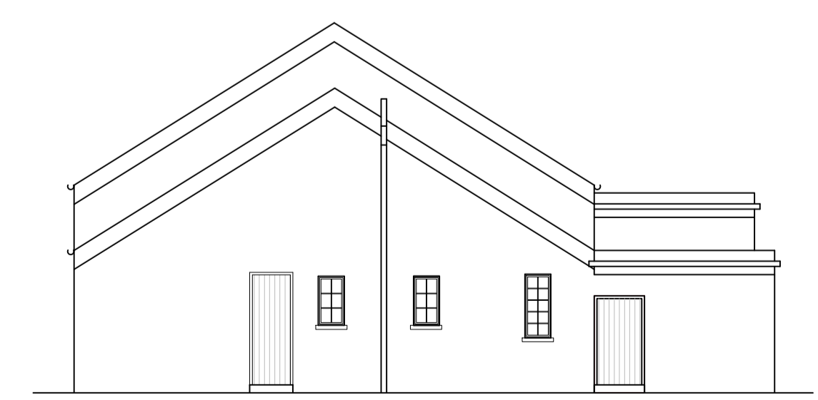
BUILDING 131 North Elevation
