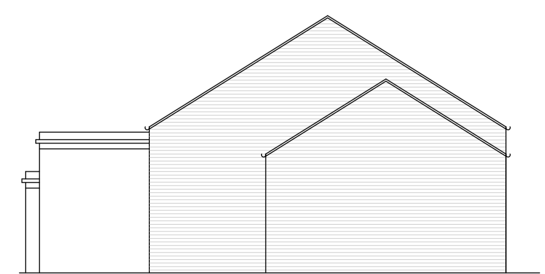
BUILDING 131 South Elevation
