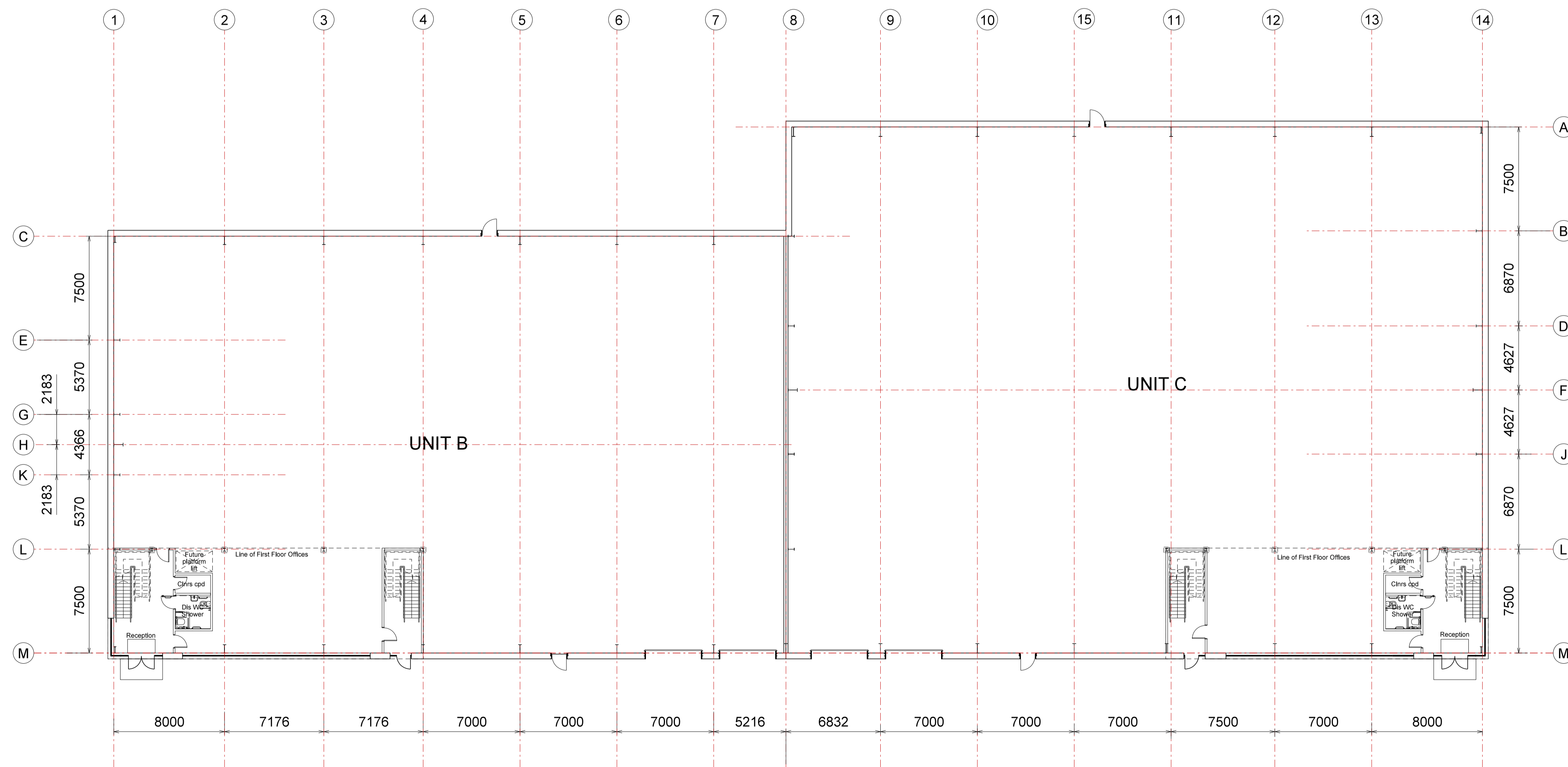
03 Ground Floor Plan 2008 Unit B & Unit C
