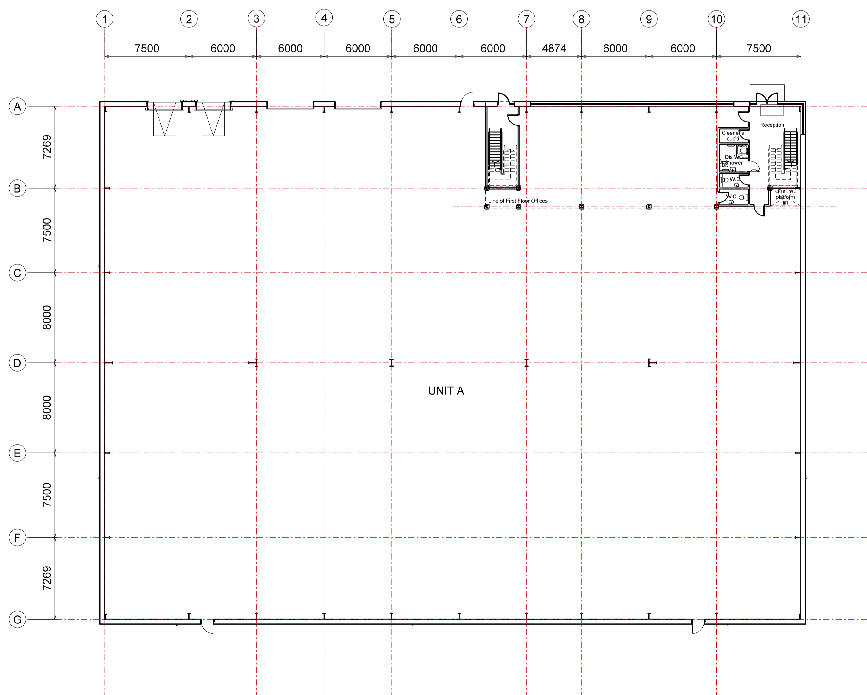
02 Ground Floor Plan 004 Unit A
