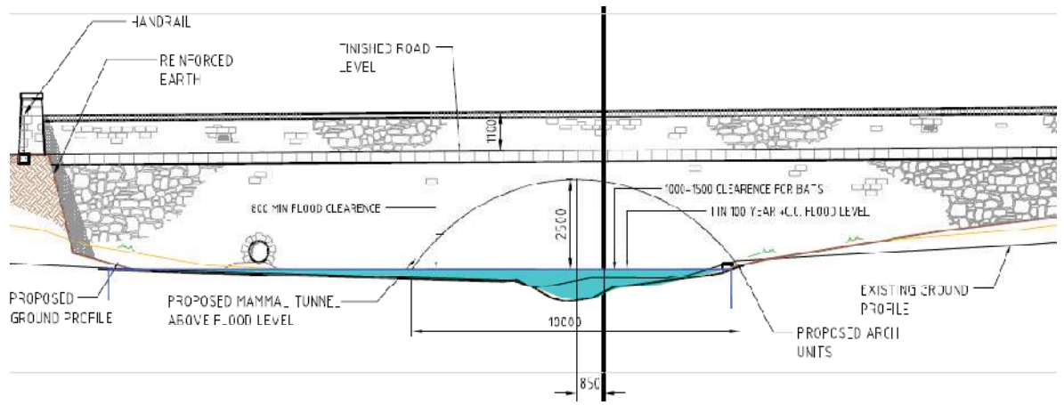
Figure 12 – Proposed downstream span bridge
