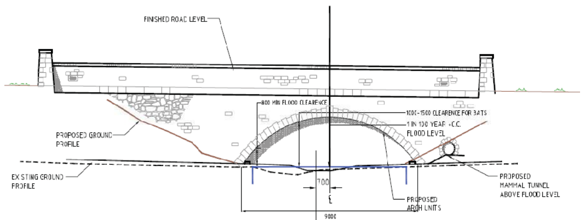
Figure 11 – Proposed upstream span bridge
