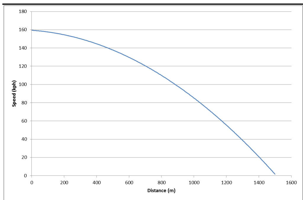
Figure 2.2 Deceleration Profile for a Class 168 DMU
