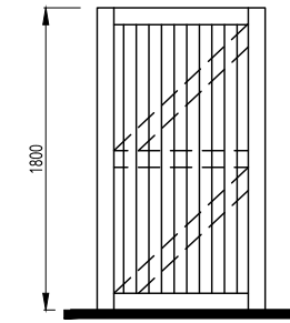
Side Access Gate 1800mm High
