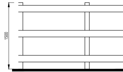
High Post & Rail Fence 1500mm High
