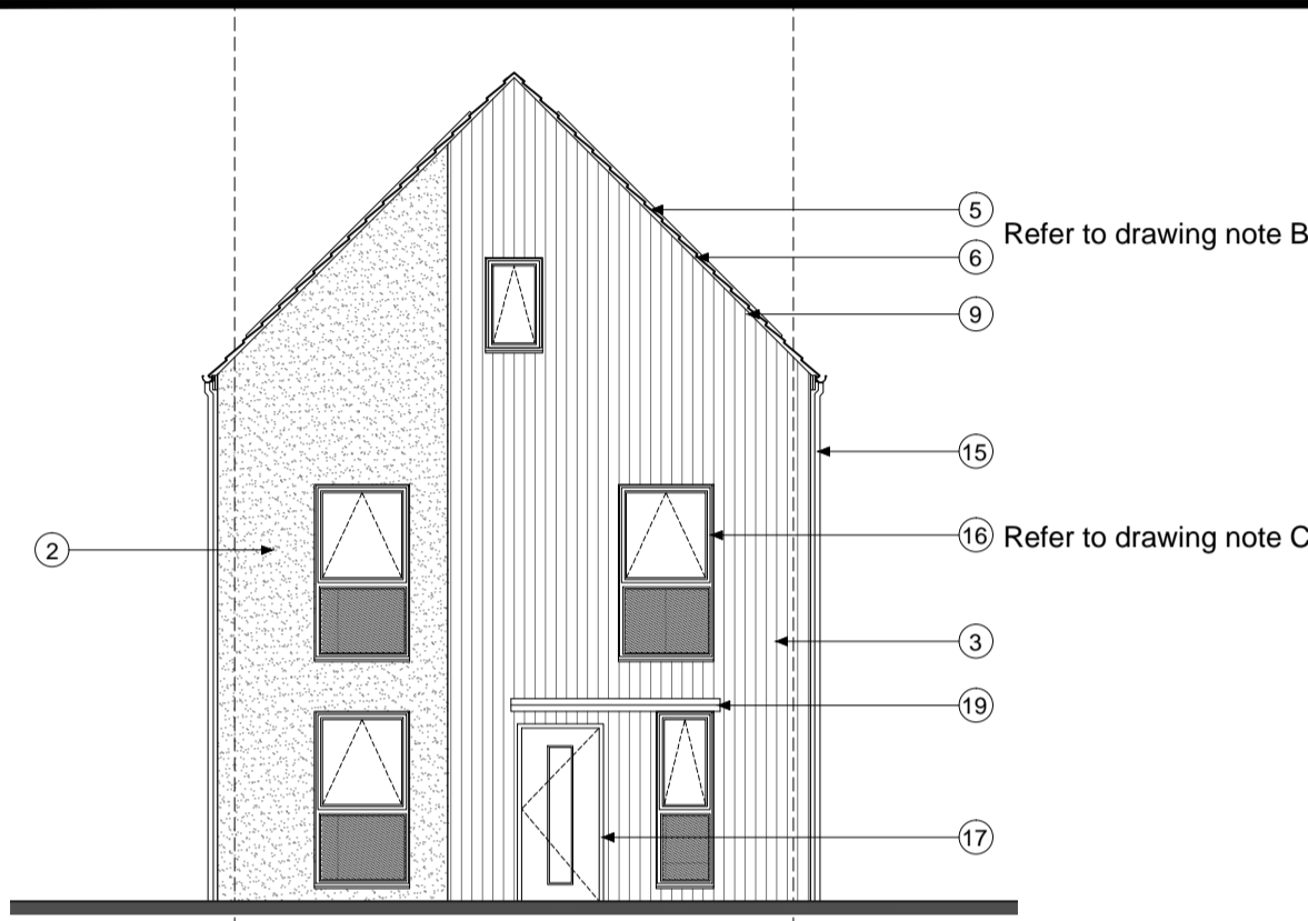
4B7P ELEVATIONS - TYPE 3 - TIMBER & RENDER - GABLE ROOF
