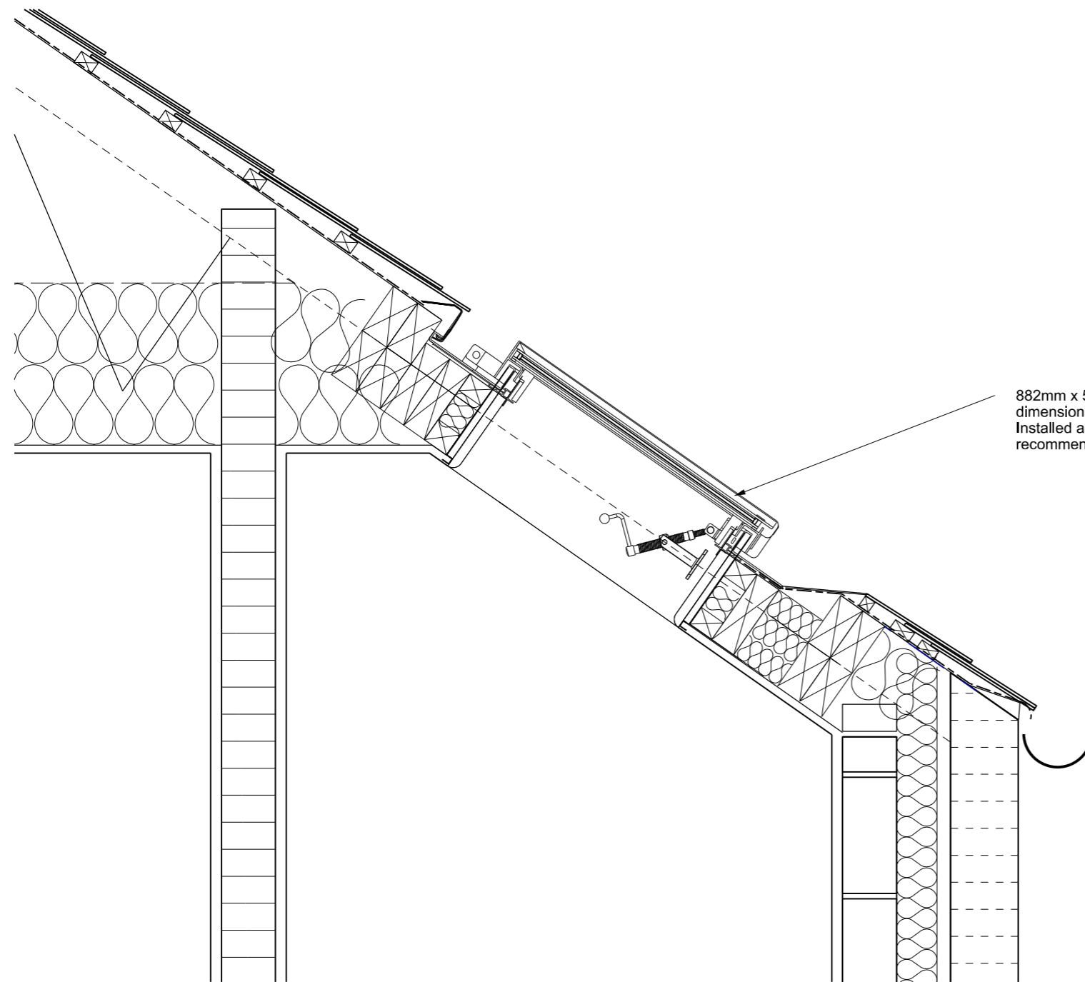
Typical section through conservation rooflight
