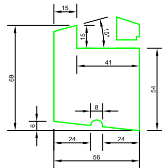
Bottom Rail S04(W) 69x56mm fin.size
