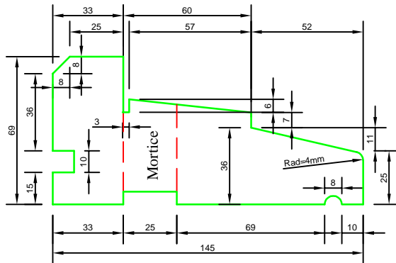
Window Cill S02(W) 145x69mm fin.size
