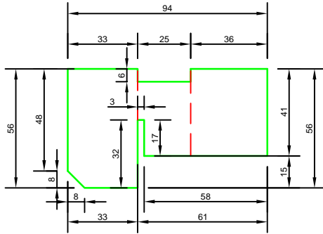
Jamb/Head Rail S01(W) 94x56mm fin.size
