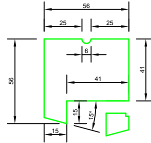
Head/Jamb S03(W) 56x56mm fin.size
