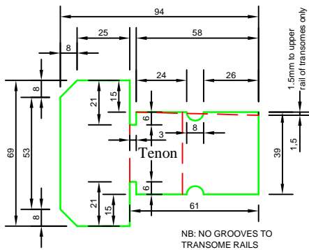
Mullion/Transome S05(W) 94x69mm fin.size
