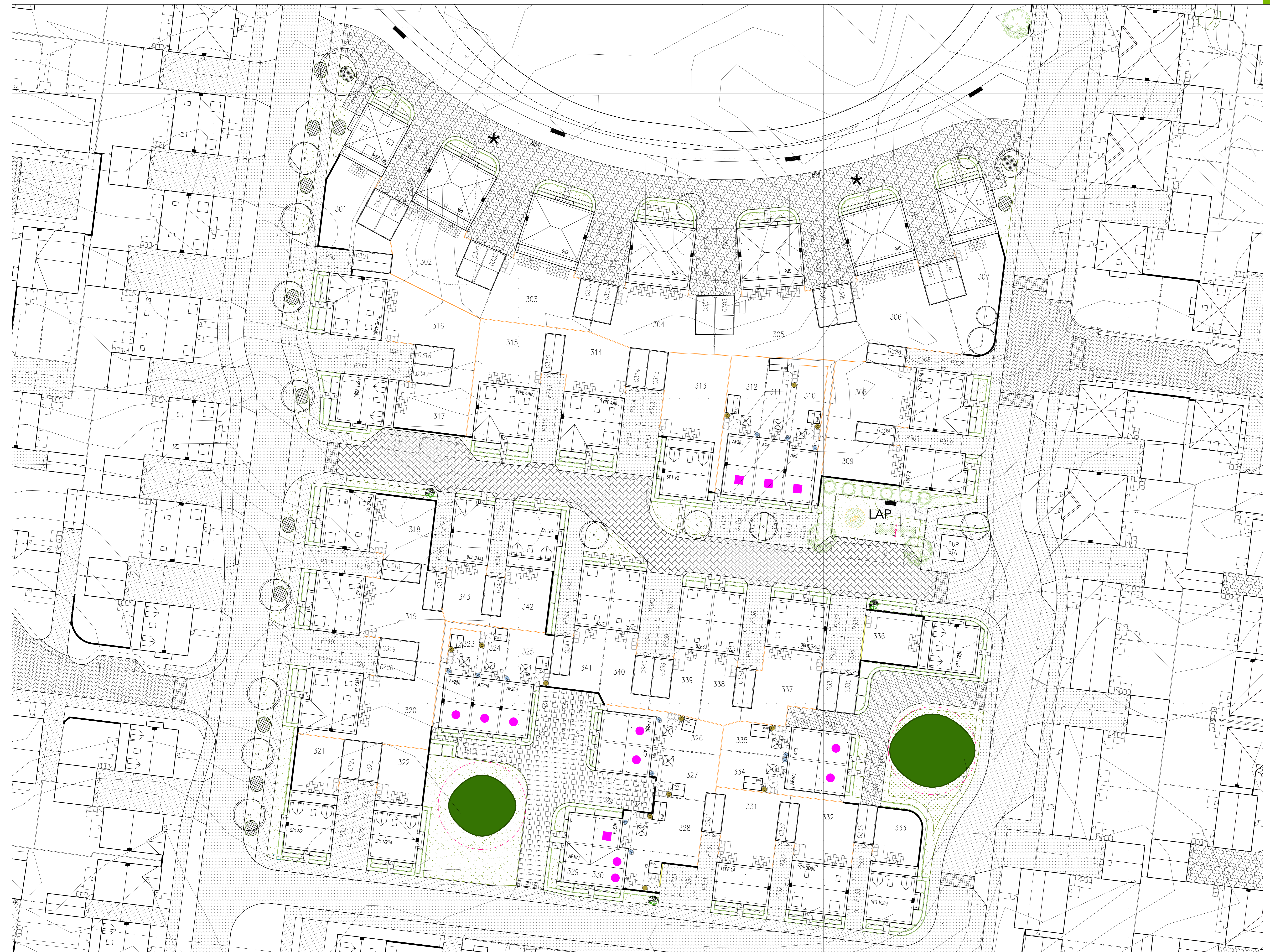
EXTERNAL WORKS LAYOUT
