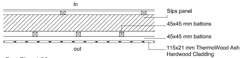
Part Plan 1:20
