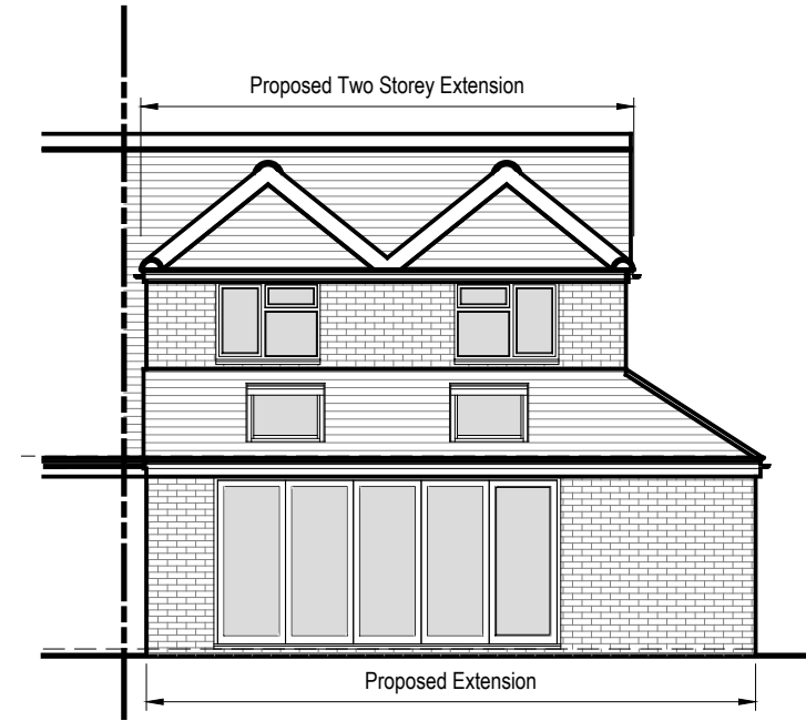
North Elevation Scale 1:100
