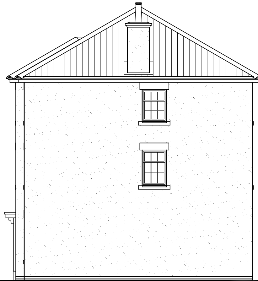
SIDE ELEVATION
