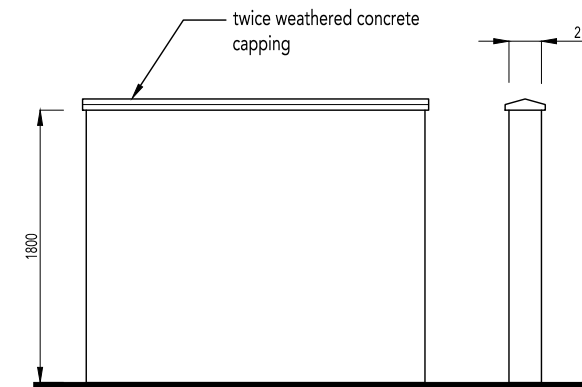
1800mm High Screen Wall
