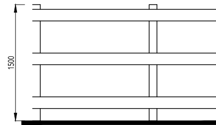
High Post & Rail Fence 1500mm High
