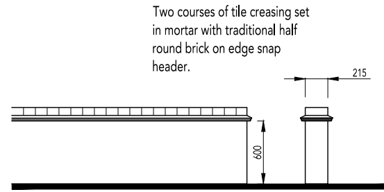
600mm High Screen Wall
