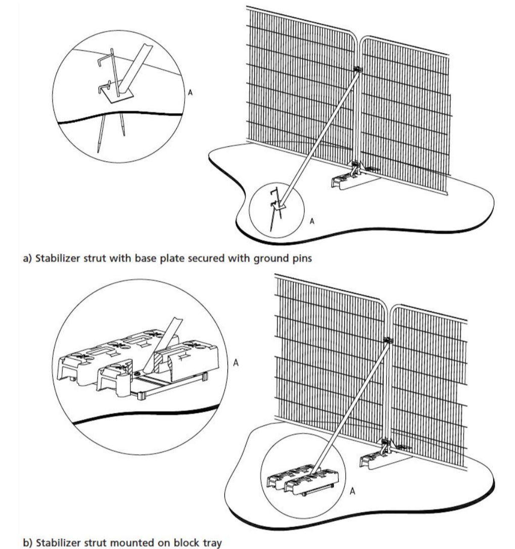
BS-5837:2012 Figure 3 Examples of above-ground stabilizing systems
