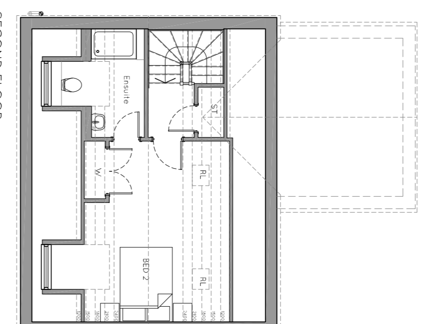
SECOND FLOOR TYPE J - BRICK PLOTS 28 & 38 READ HANDED
