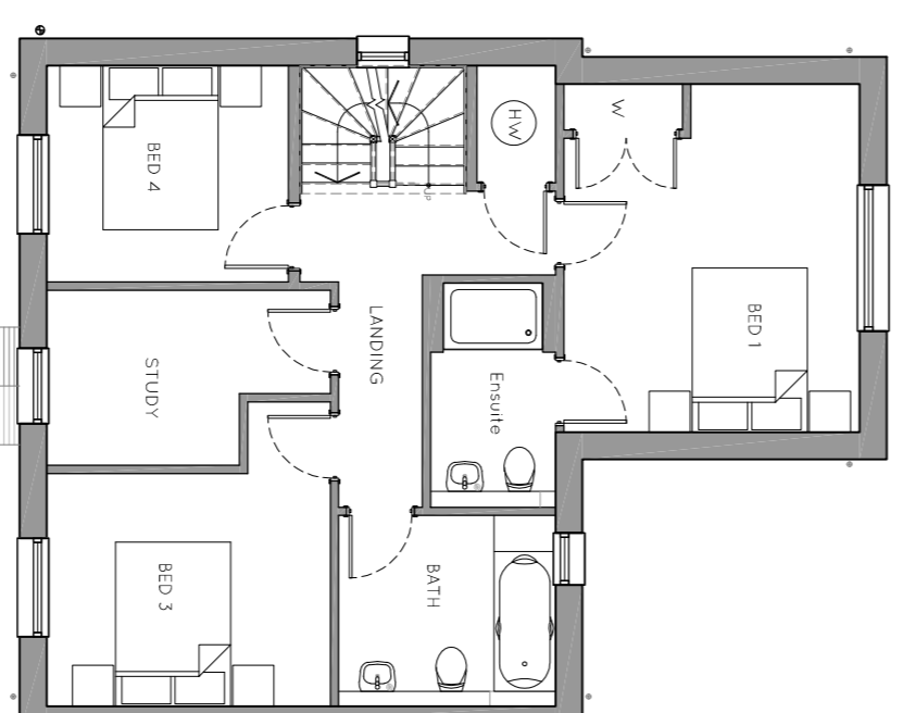
FIRST FLOOR TYPE J - BRICK PLOTS 28 & 38 READ HANDED
