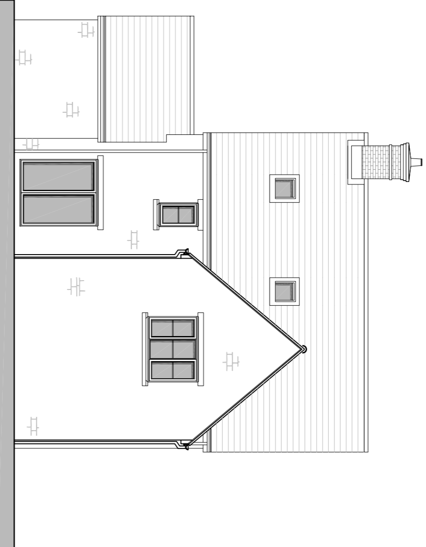
REAR ELEVATION TYPE J - IRON STONE PLOT 61 (PLOTS 37 & 62 READ AS HANDED)
