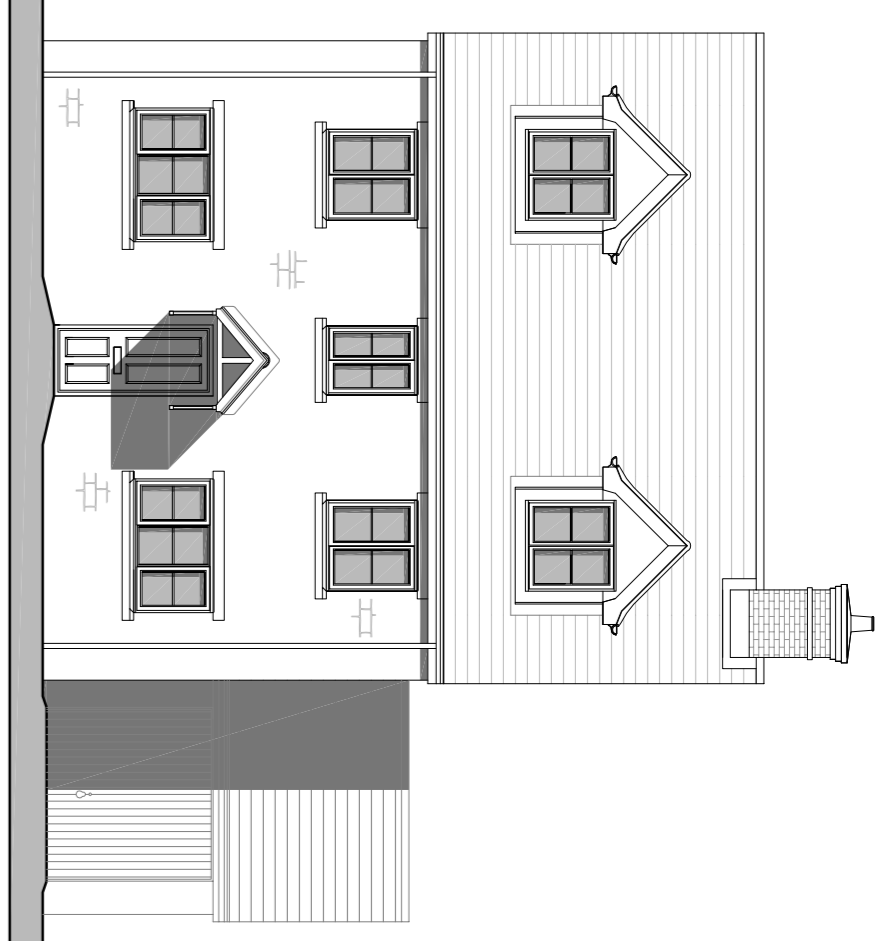
FRONT ELEVATION TYPE J - IRON STONE PLOT 61 (PLOTS 37 & 62 READ AS HANDED)
