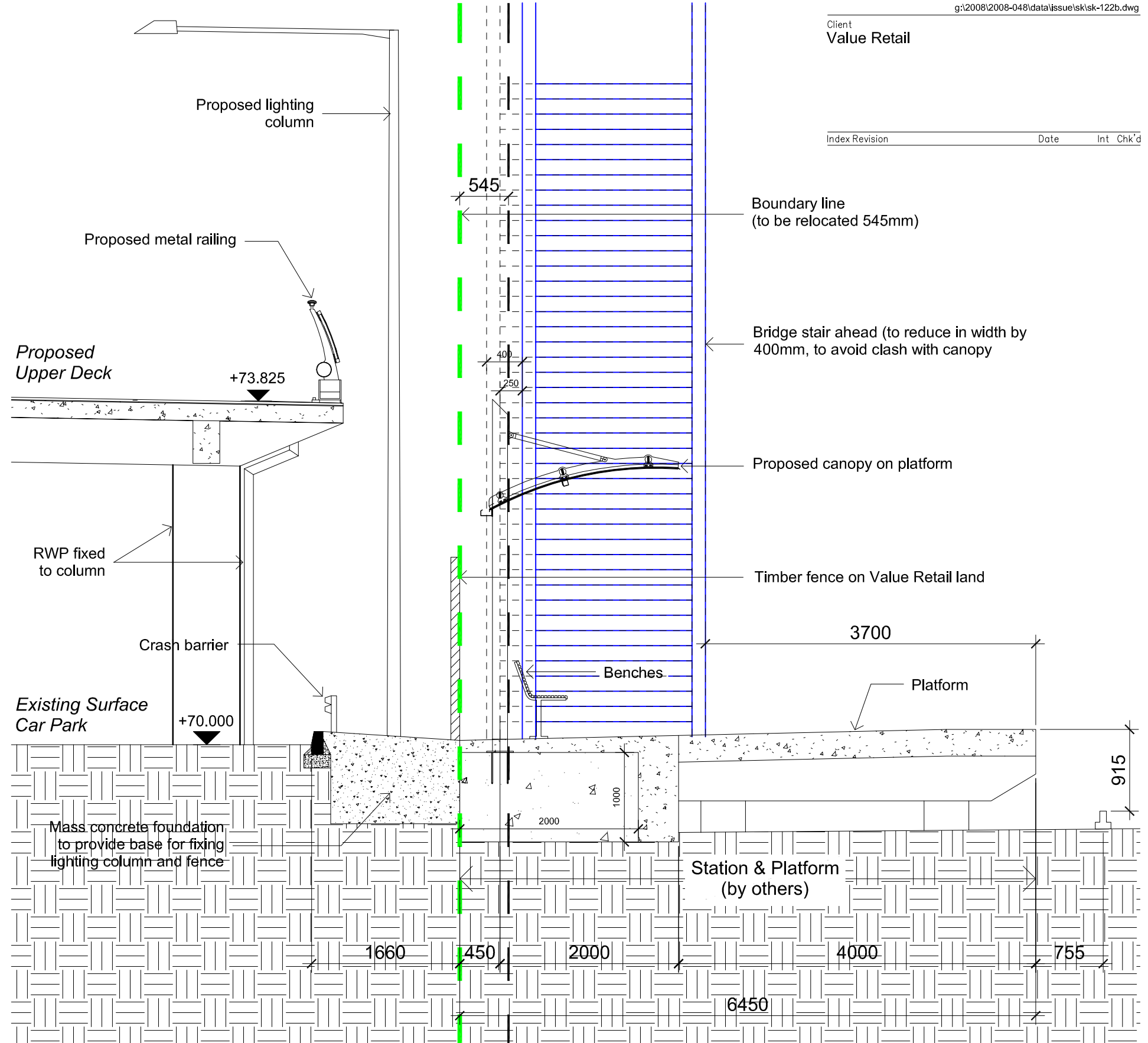
SK-122 - Platform Boundary Section (1:50)
