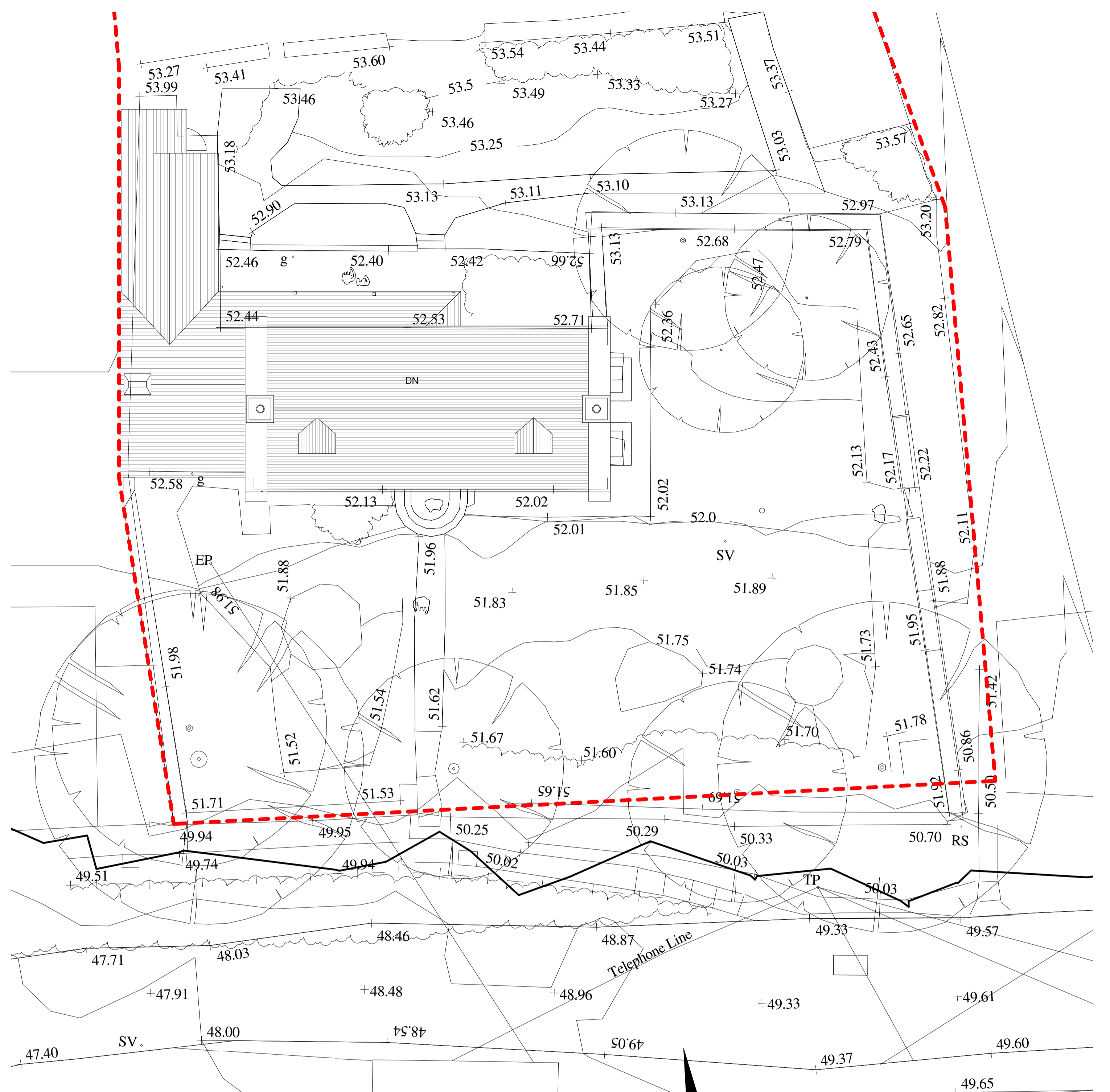
Topographical Survey
