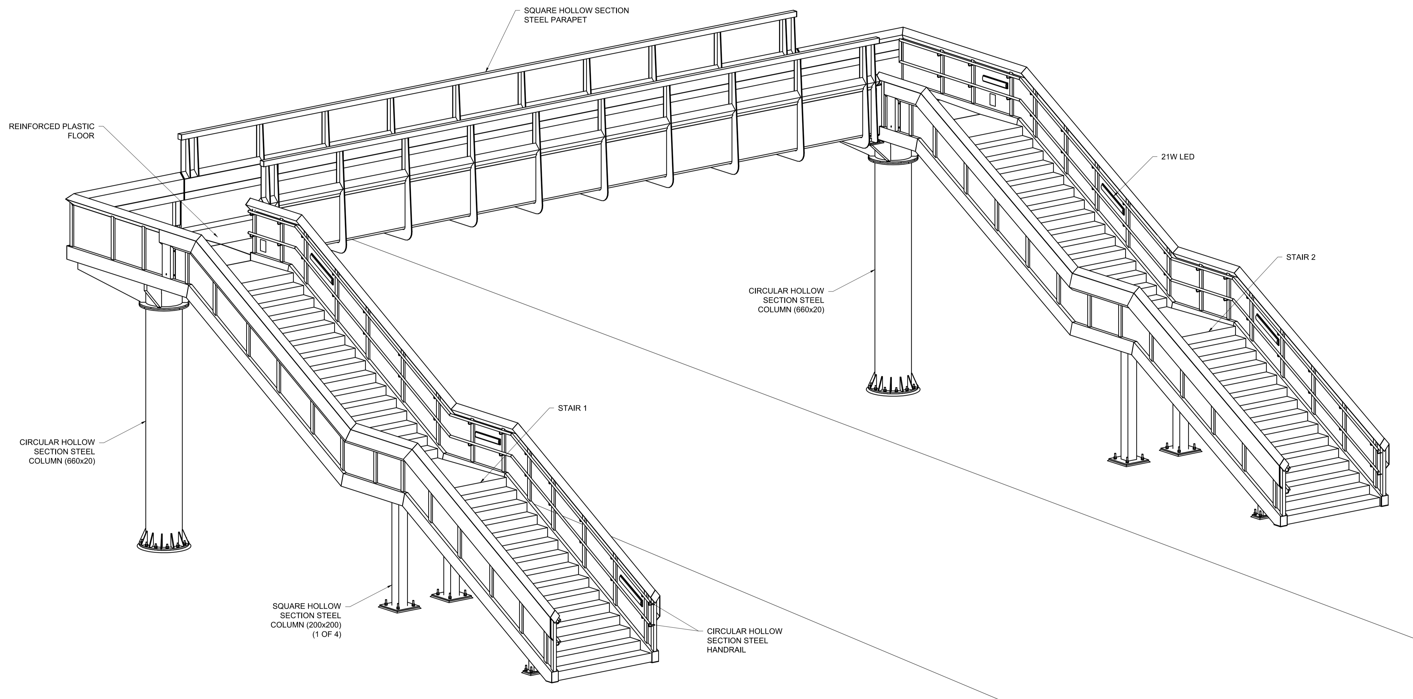
ISOMETRIC VIEW NTS
