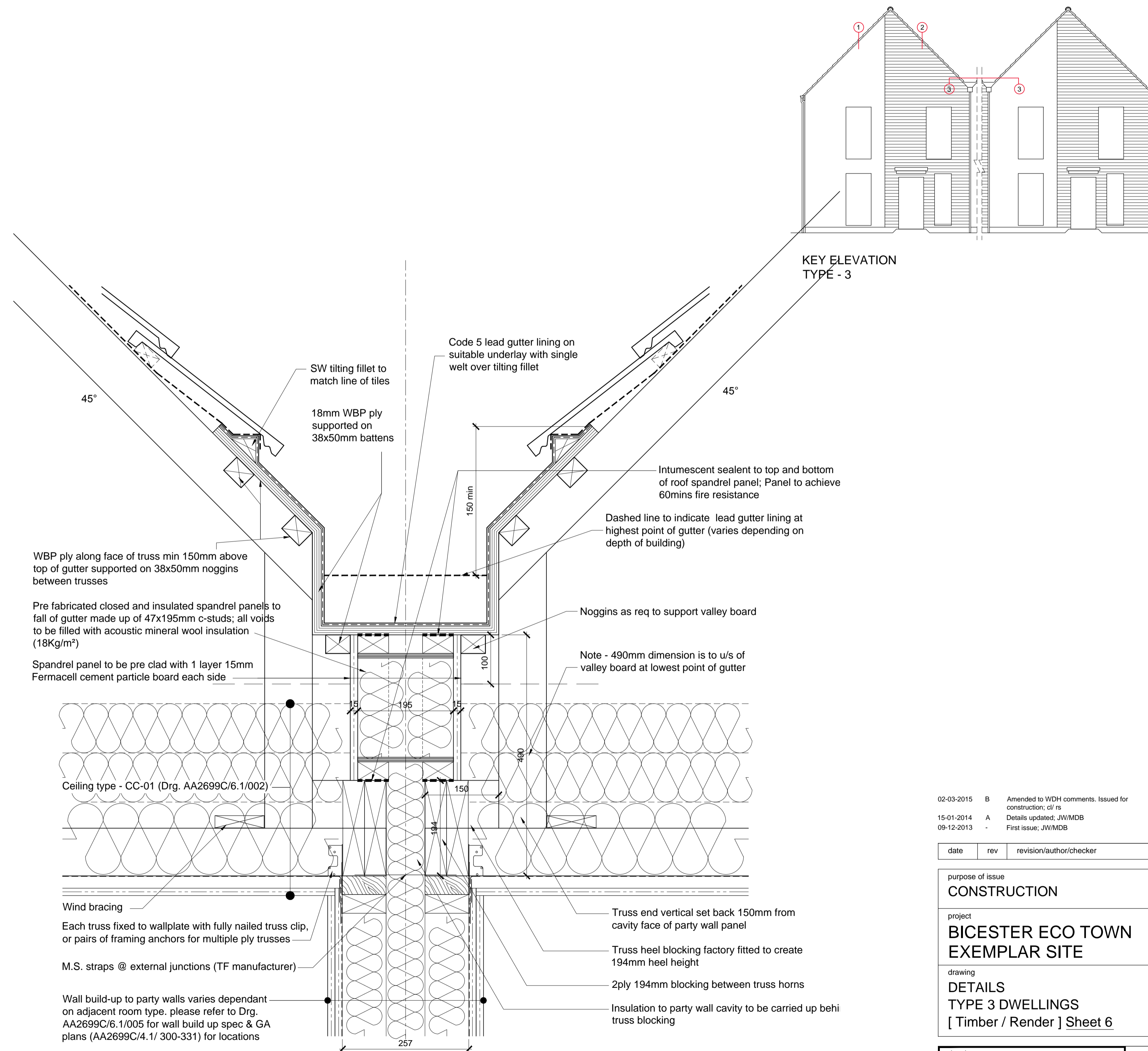
03 Secret Gutter Detail Type 3 - Timber / Render
