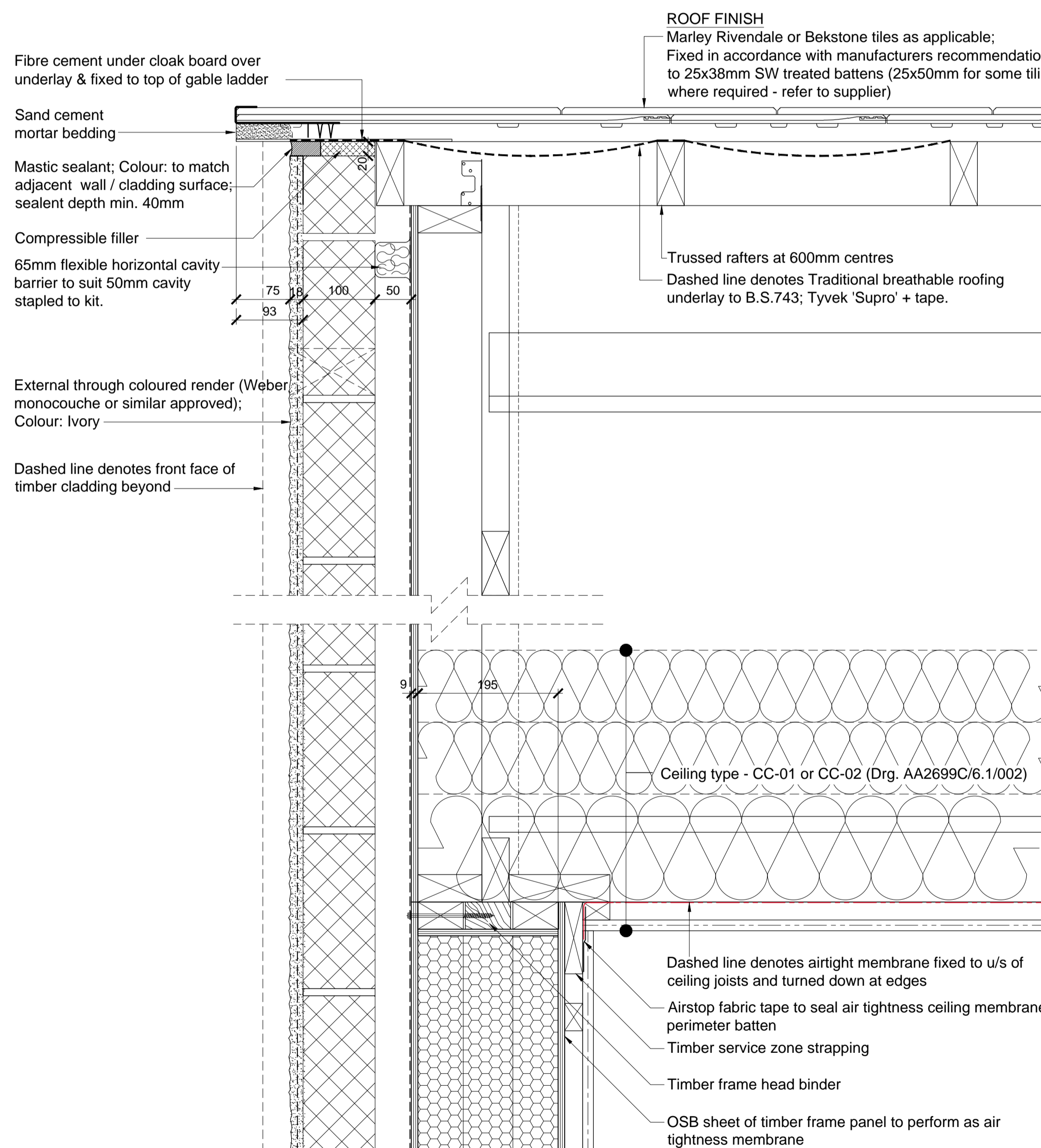
02 Verge Detail (Timber) Type 3 - Timber / Render
