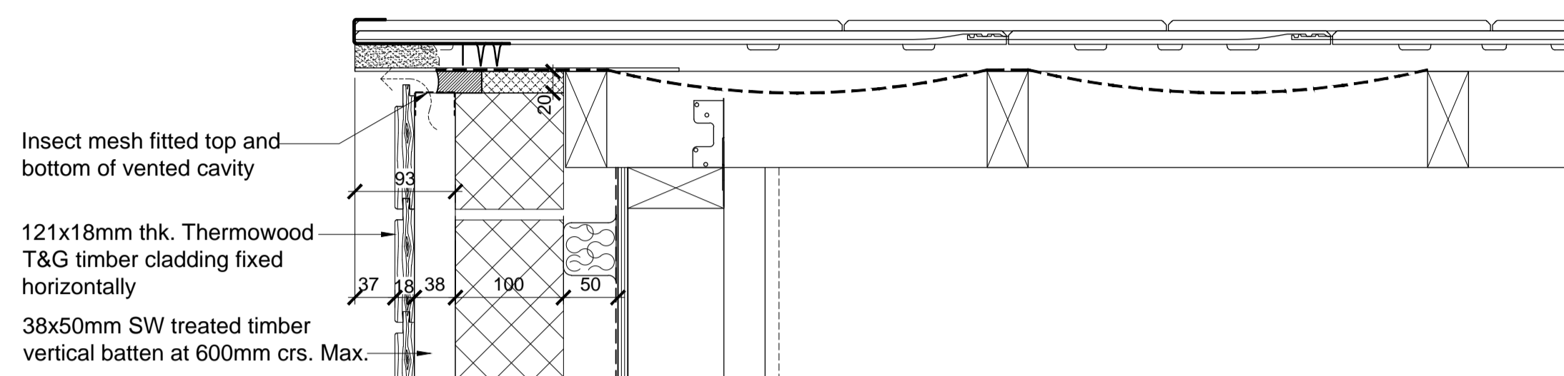
02 Verge Detail (Timber) Type 3 - Timber / Render
