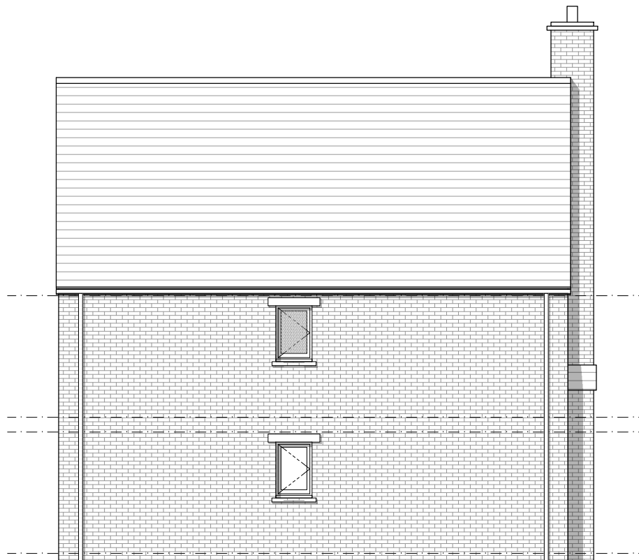
Front Elevation - D2 1:100 (A3)
