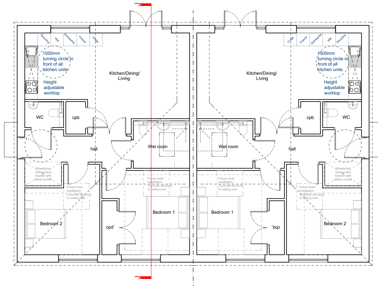
Floor Plan - BuBu 1:100 (A3)
