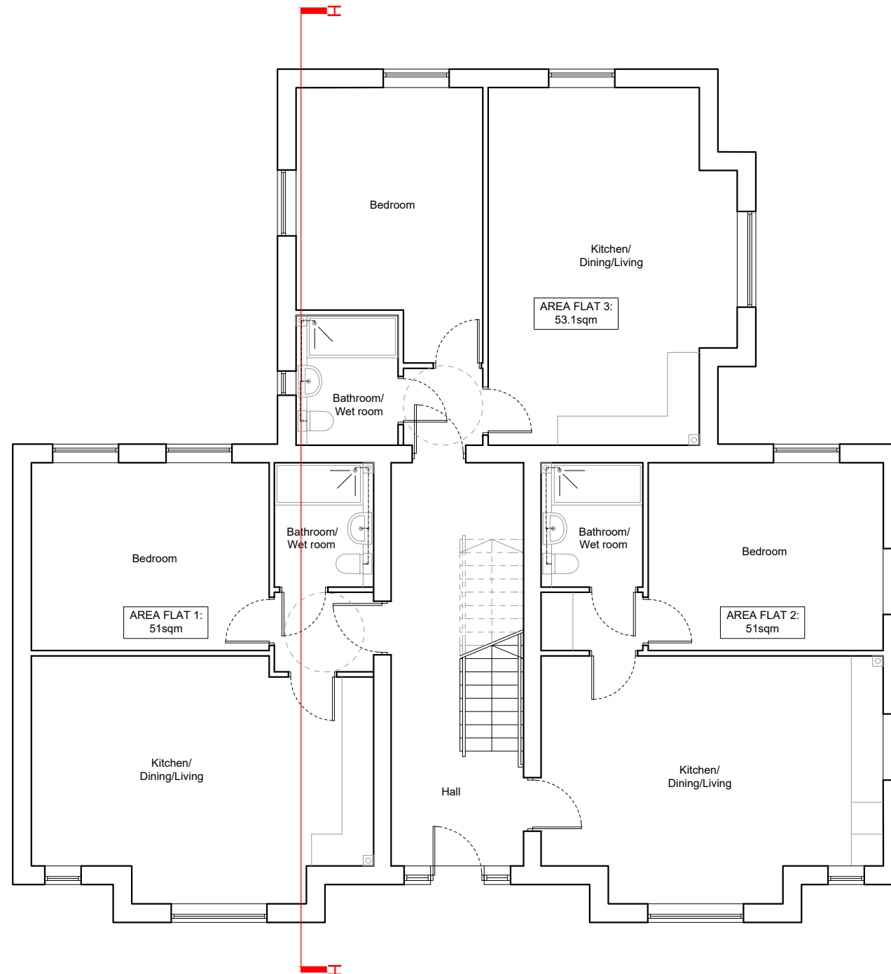
Ground Floor Plan - 6xF 1:100 (A3)
