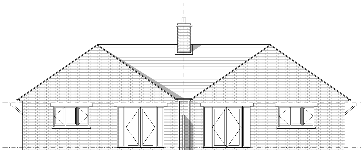
Rear Elevation - BuBu 1:100 (A3)
