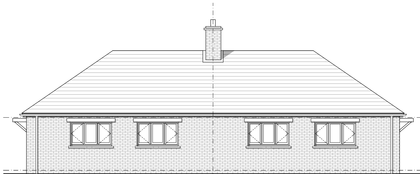
Front Elevation - BuBu 1:100 (A3)
