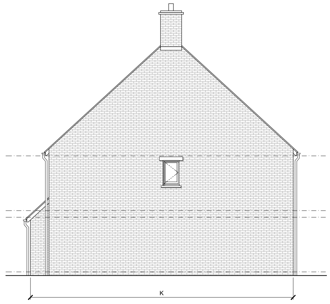
Side Elevation - K 1:100 (A3)
