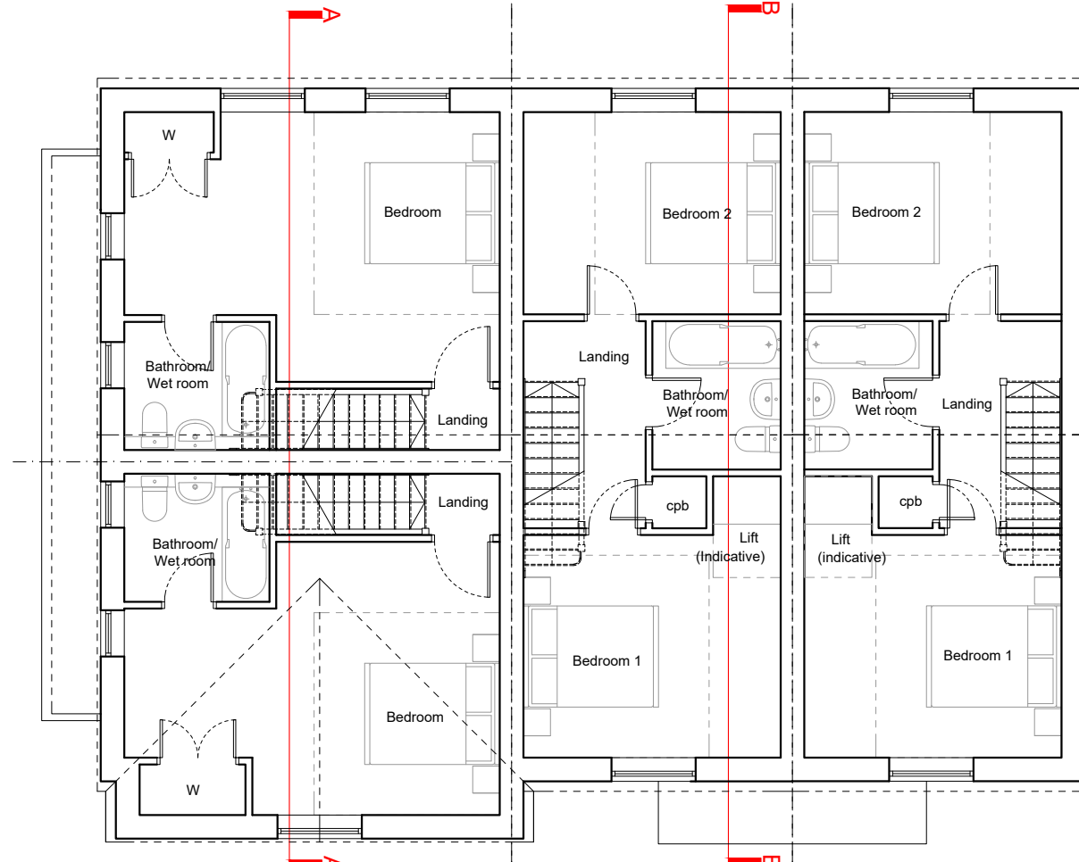
First Floor Plan - KeKeKK 1:100 (A3)
