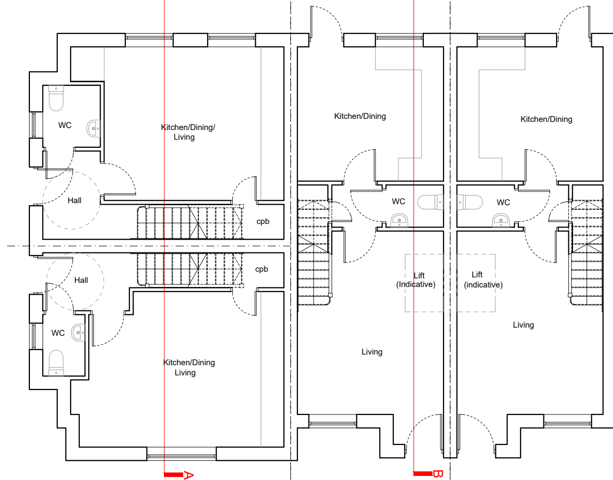
Ground Floor Plan - KeKeKK 1:100 (A3)
