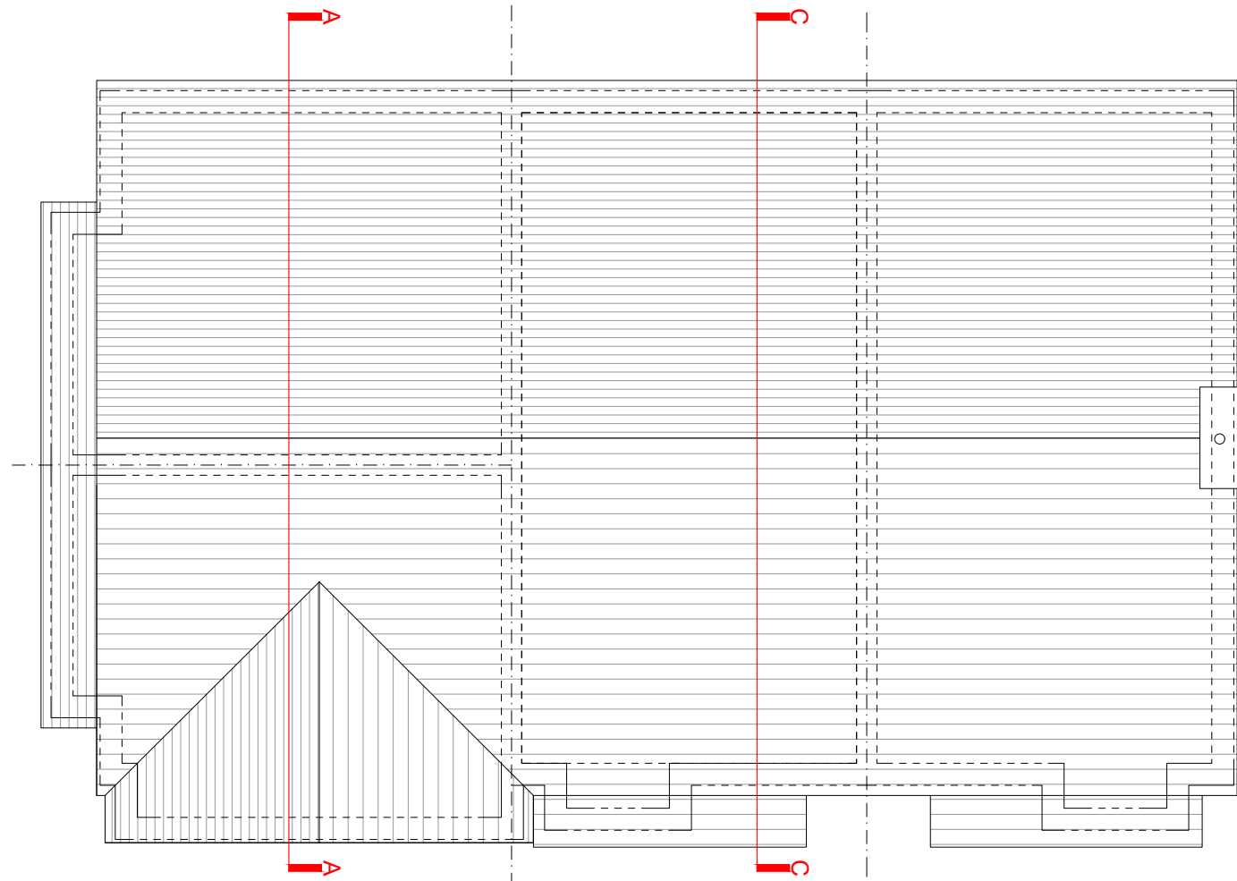
Roof Plan - KeKeBB 1:100 (A3)
