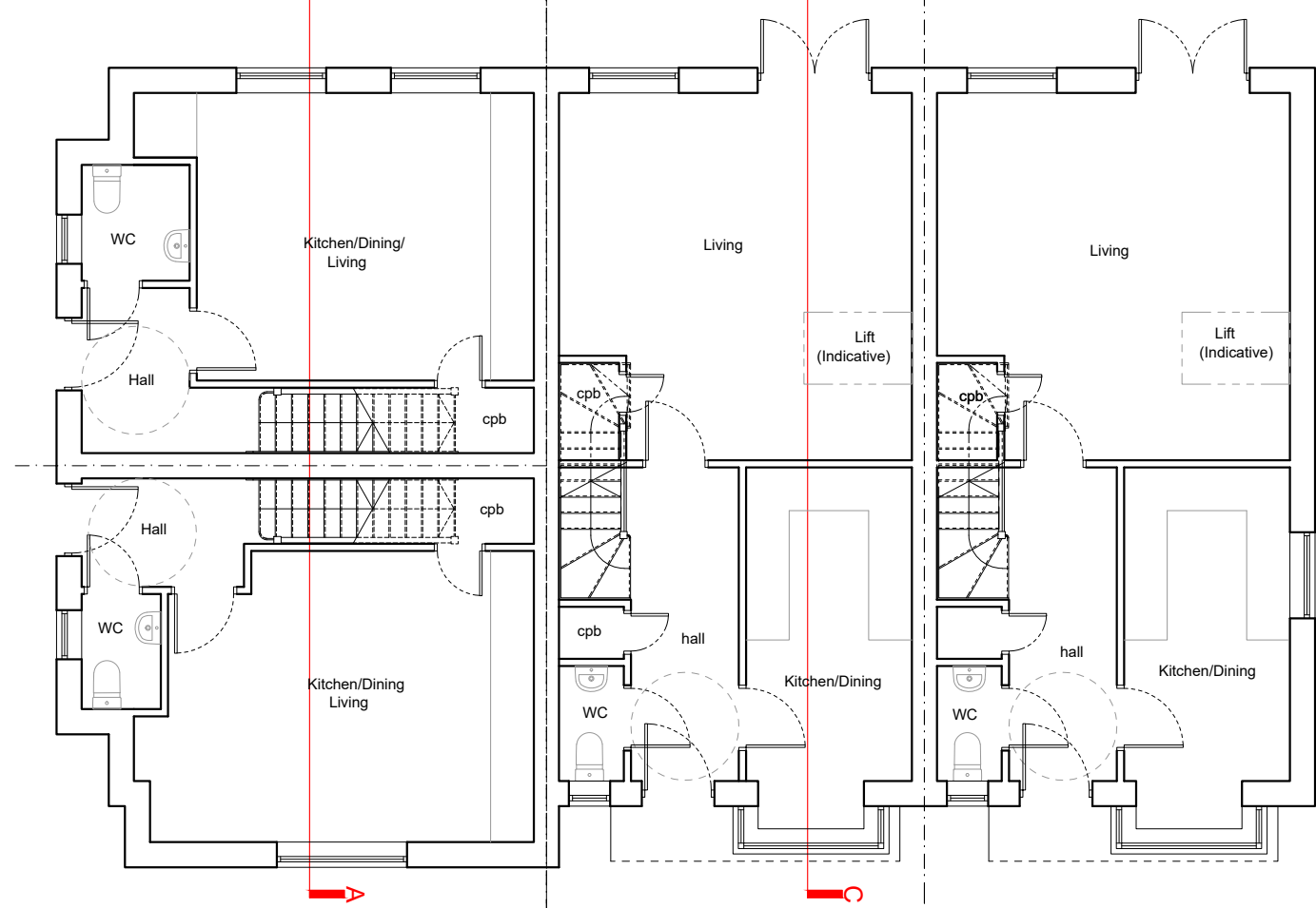
○ Ground Floor Plan - KeKeBB 1:100 (A3)
