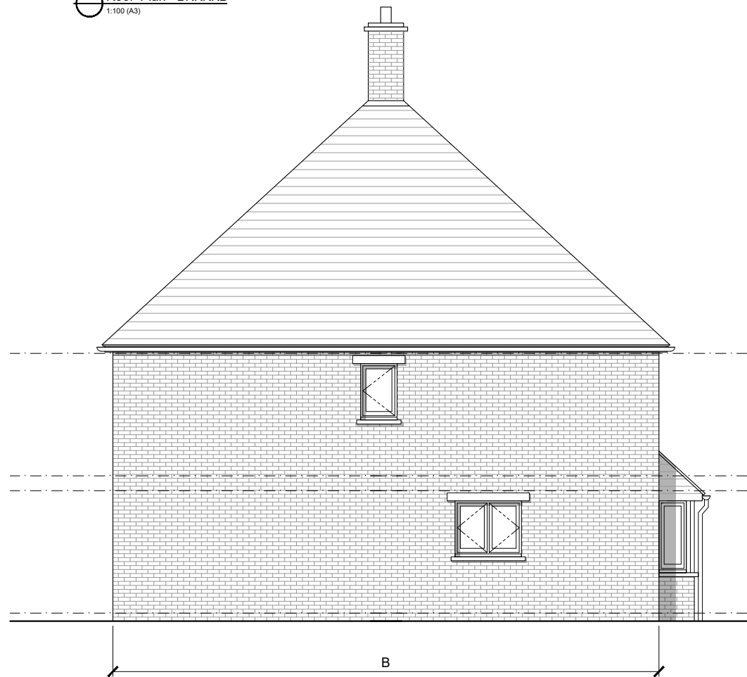
Side Elevation - BKKKKB 1:100 (A3)
