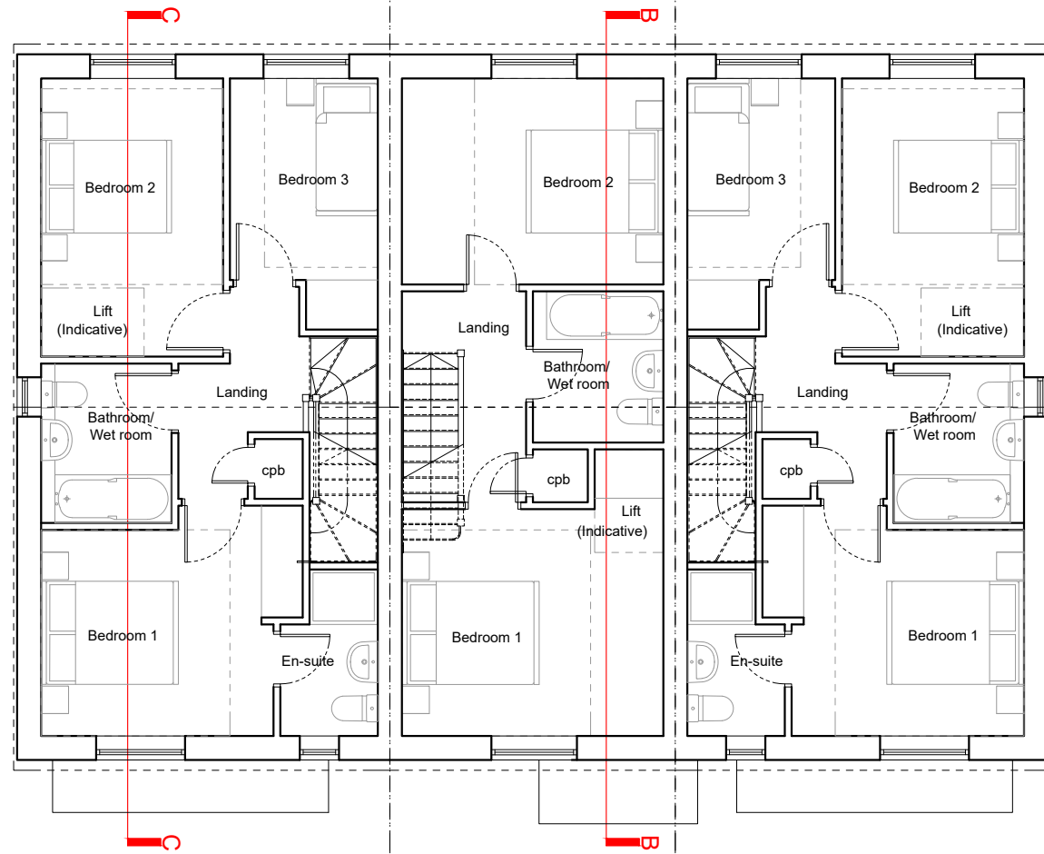
First Floor Plan - BKB 1:100 (A3)
