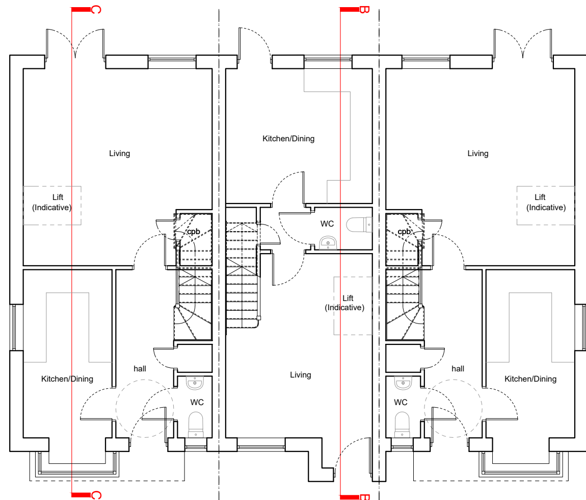
Ground Floor Plan - BKB 1:100 (A3)
