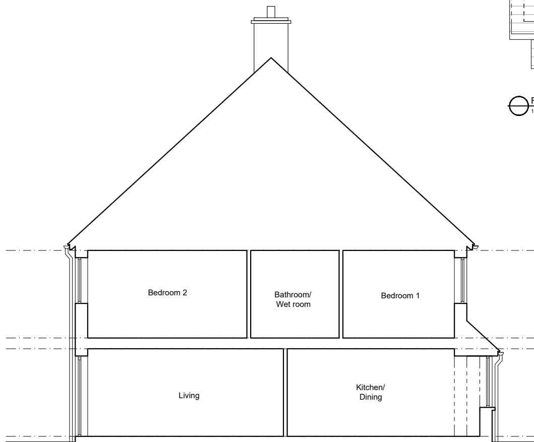
Section CC 1:100 (A3)
