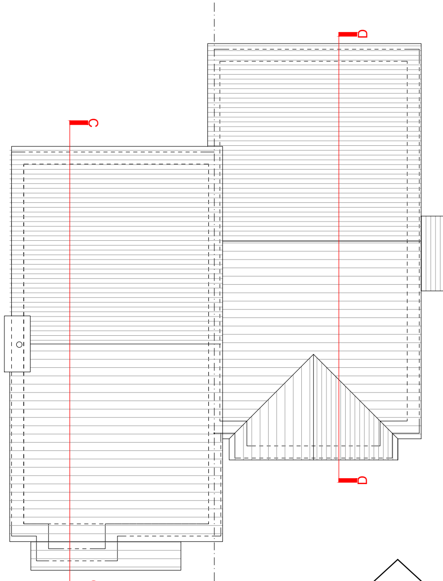
Roof Plan - BR 2 1:100 (A3)
