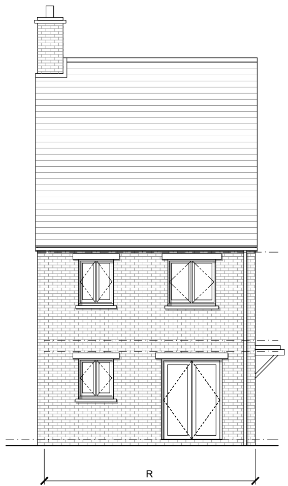
Rear Elevation - R 1:100 (A3)
