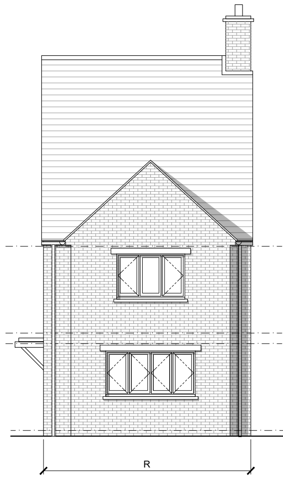
Front Elevation - R 1:100 (A3)
