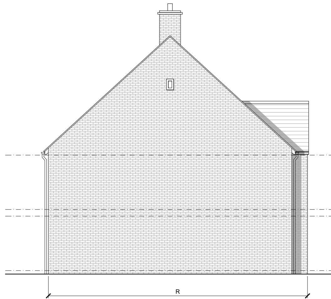
Side Elevation 2 - R 1:100 (A3)
