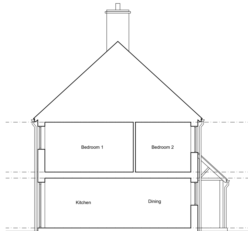
Section FF 1:100 (A3)
