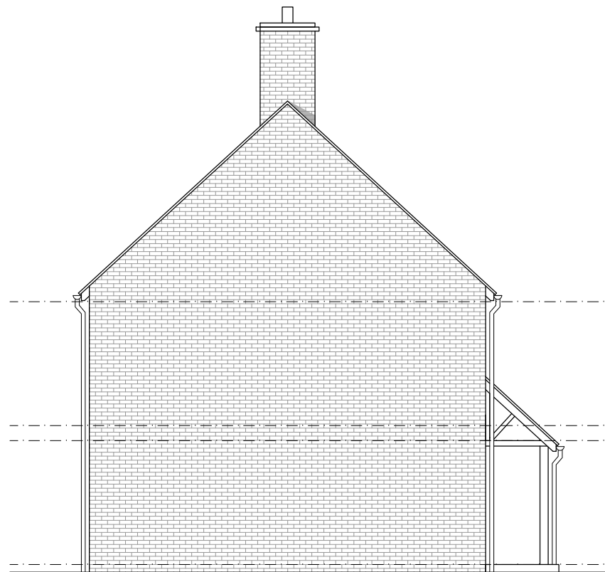
Side Elevation - W 1:100 (A3)
