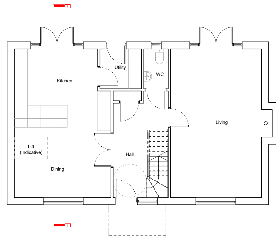
○ Ground Floor Plan - W 1:100 (A3)
