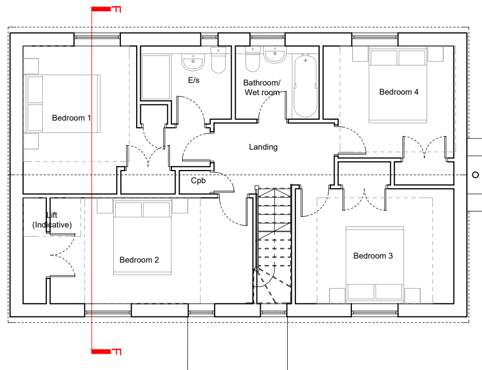
○ First Floor Plan - W 1:100 (A3)
