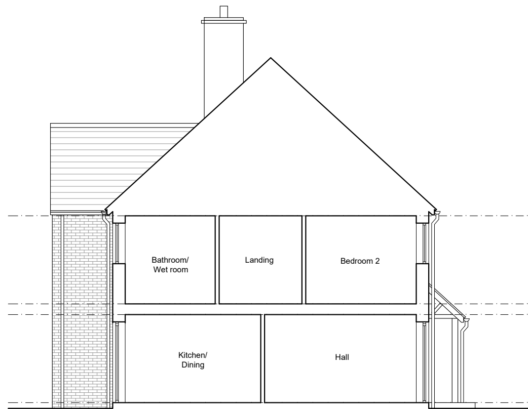
Section EE 1:100 (A3)
