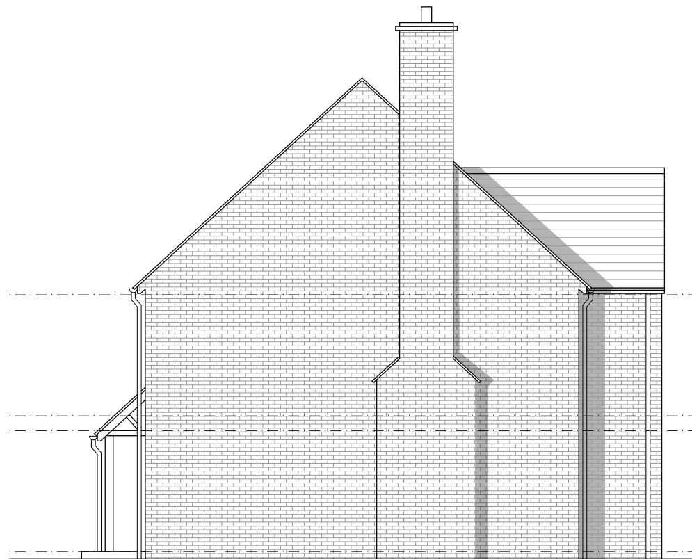
Side Elevation - D 1:100 (A3)
