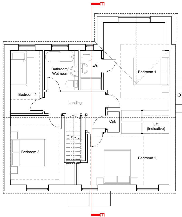
First Floor Plan - D 1:100 (A3)
