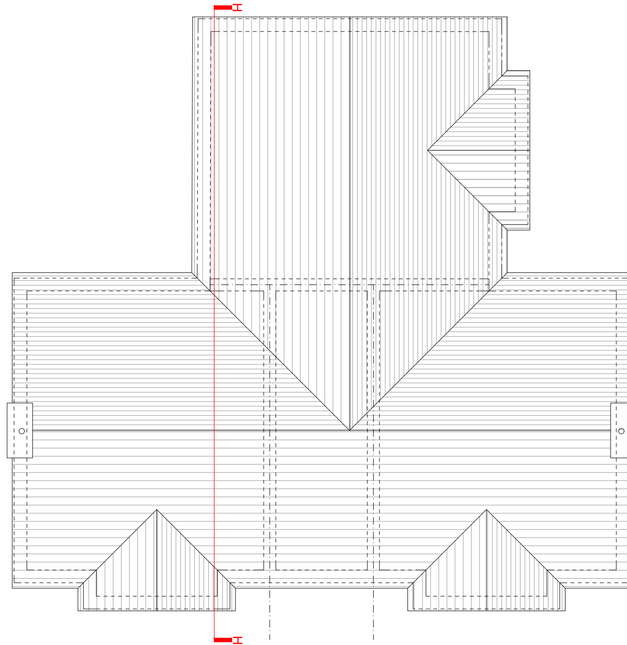
Roof Plan - 6xF 1:100 (A3)
