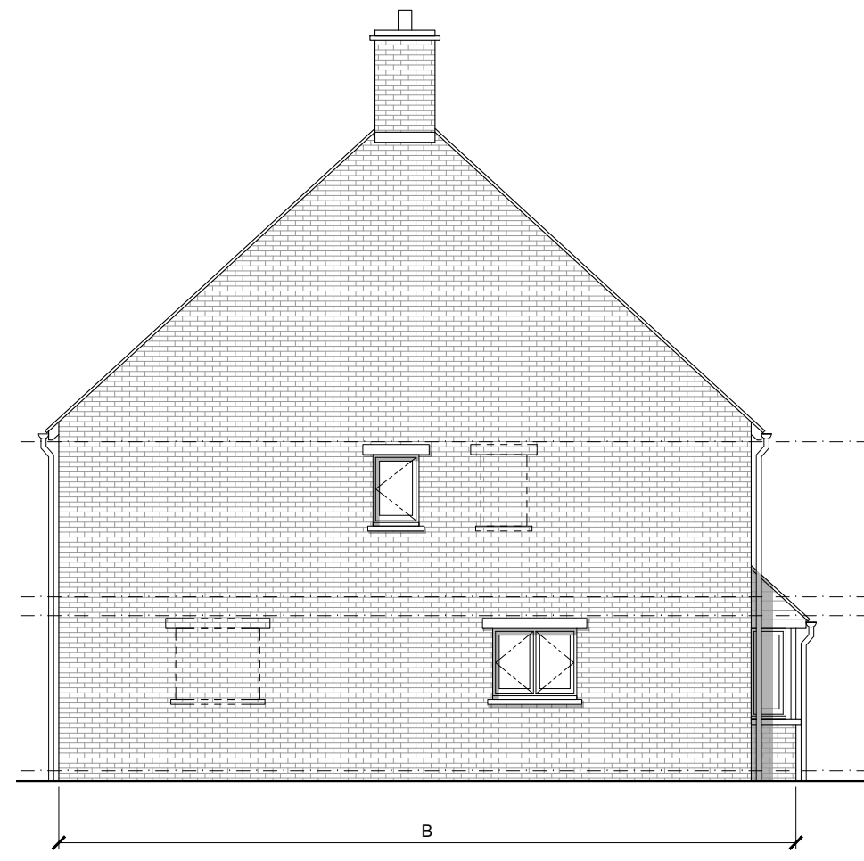
Side Elevation - B 1:100 (A3)
