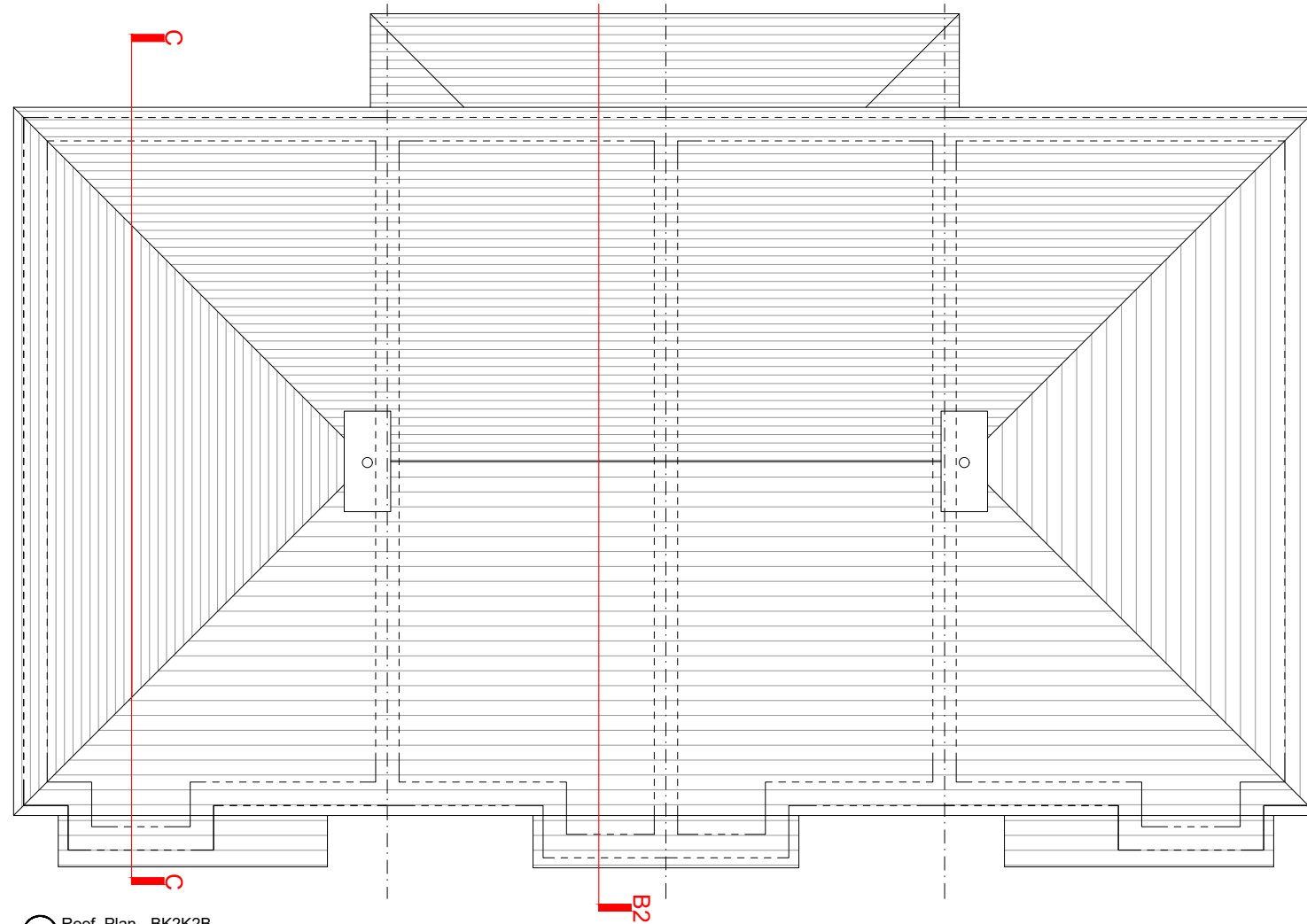
Roof Plan - BK2K2B 1:100 (A3)
